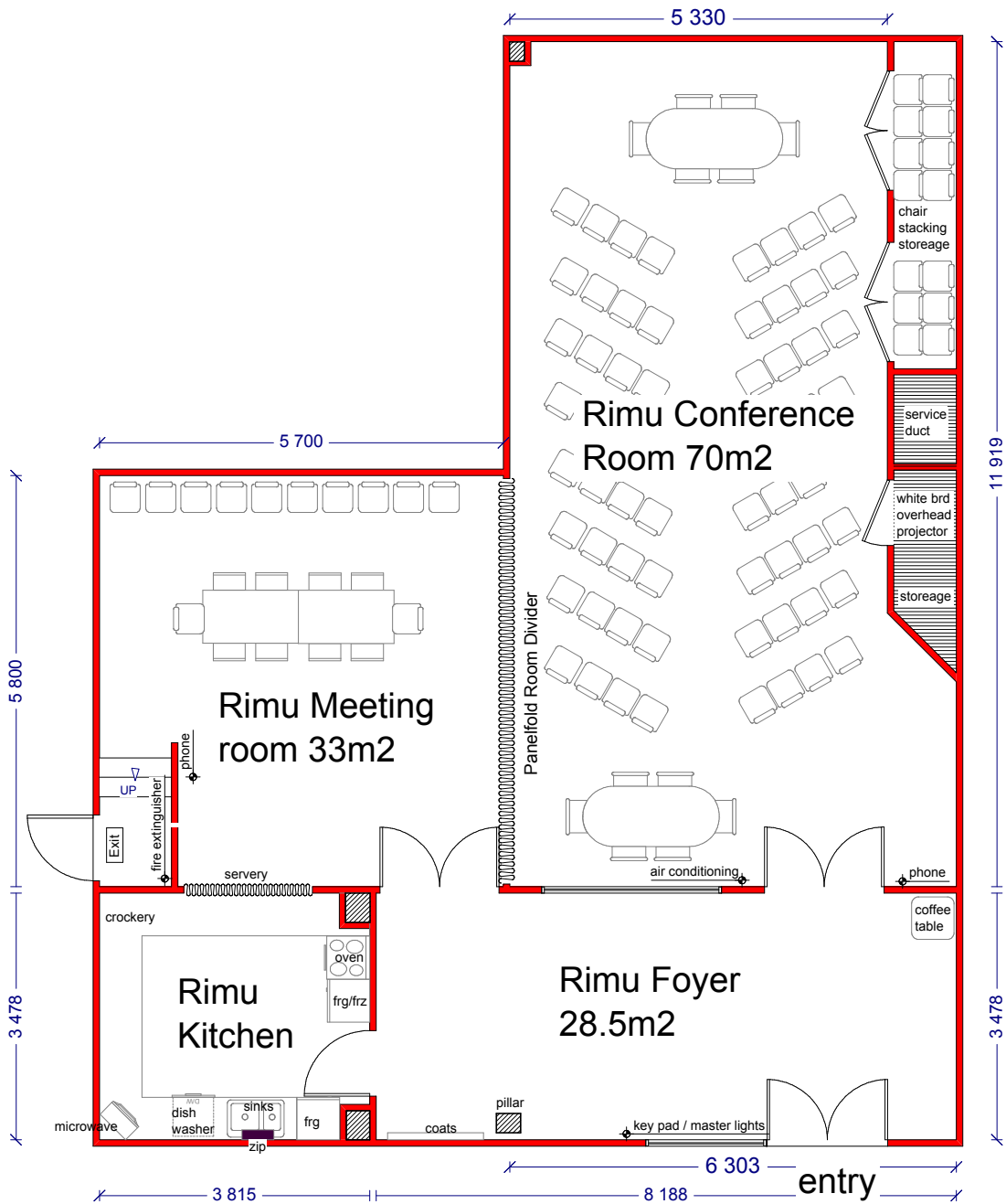
floor plan 1:100 Tenancy 109 "Rimu Rooms"
